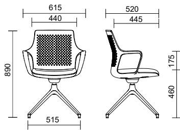
MEETING WITH 4 STAR BASE AND WITH TILTING SYSTEM
