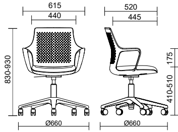
MEETING WITH 5 STAR BASE, ADJUSTABLE IN HEIGHT
