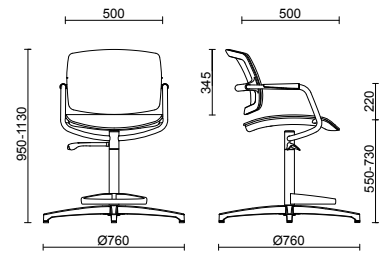
STOOL SEAT HEIGHT ADJUSTABLE
