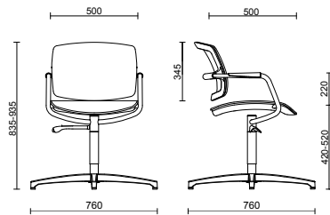
MEETING WITH SEAT AND BACK IN MESH
