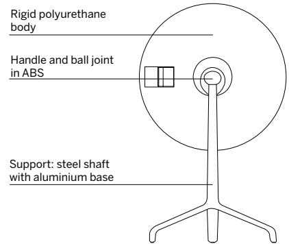
USEME STANDARD - BACK
